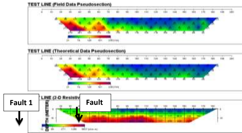
Figure 4b: Dipole-dipole pseudo section for Traverse 1
