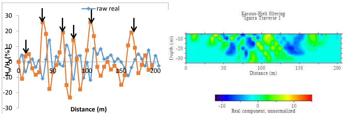
Figure 4a: (VLF) profile and pseudo-section for Traverse 1
